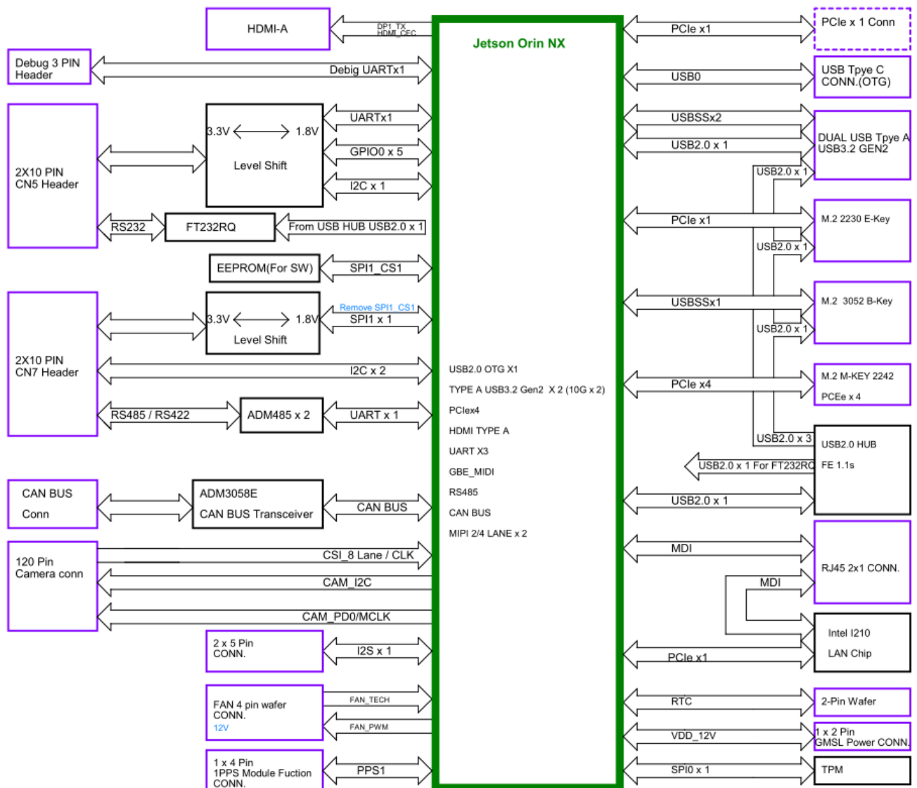
AIB-MO22/32 & AIB-MN32/42-S2 Block diagram
